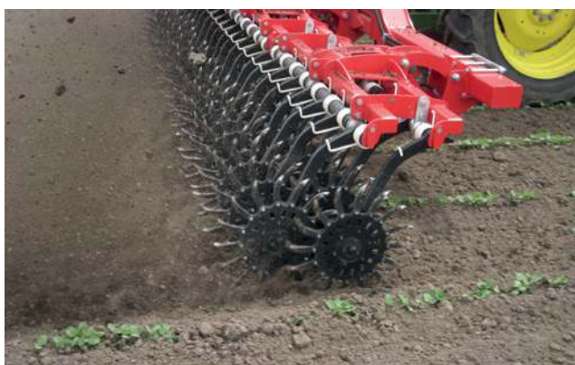
Rotary hoes can be operated at high speeds
